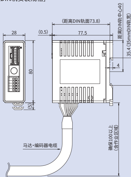
[DIN轨安装规格]
